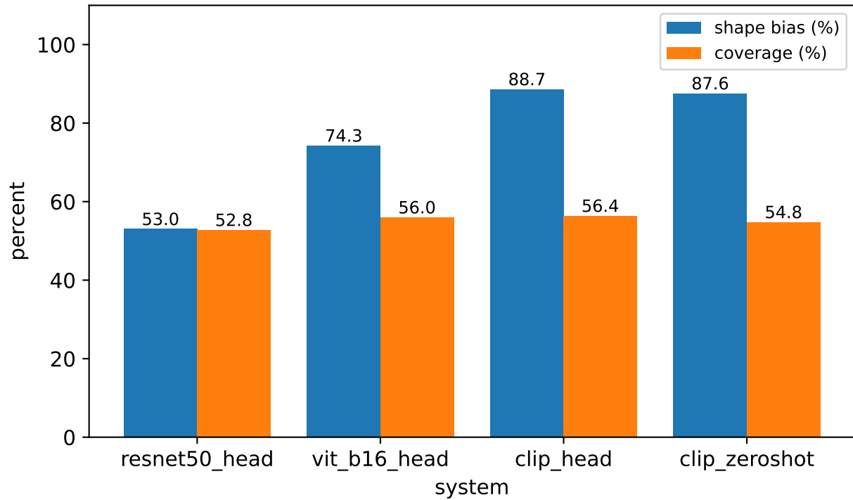
Shape bias with coverage
