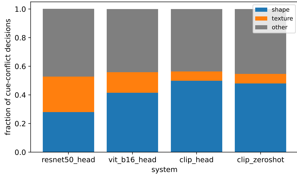
Decisions on 250 cue conflicts
