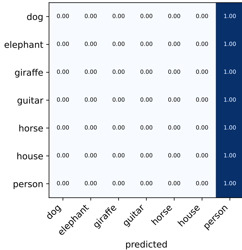
DAN-DG ( \lambda=1 ) (Sketch acc 0.041)
