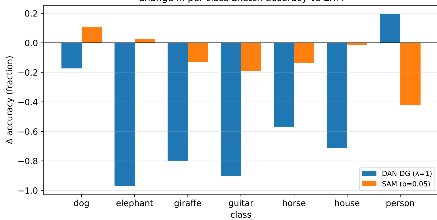
Change in per-class Sketch accuracy vs ERM
