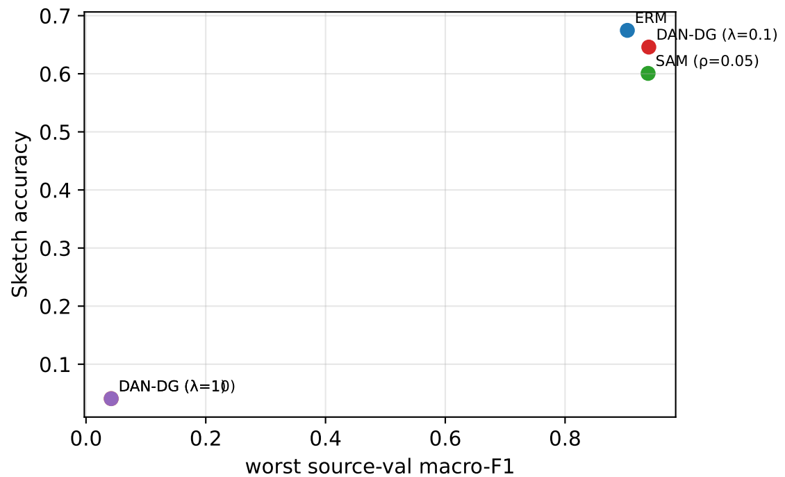
Source-side validation vs unseen-domain (Sketch) accuracy
