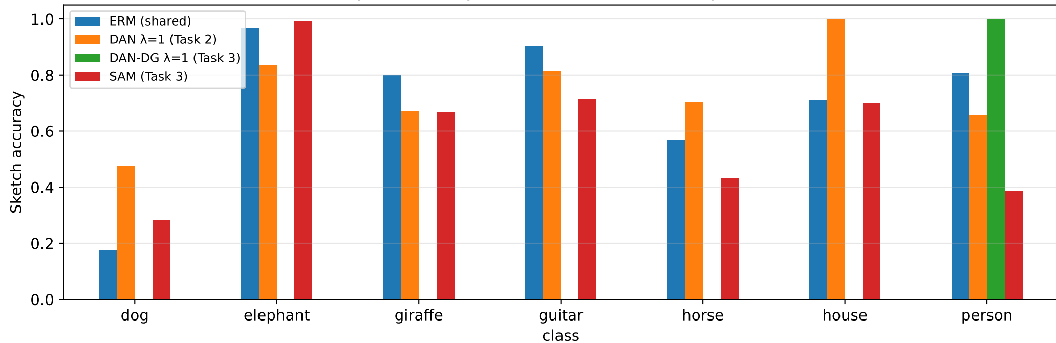
Per-class Sketch accuracy: ERM vs target-aware DAN (Task 2) vs target-free DAN-DG / SAM (Task 3)
