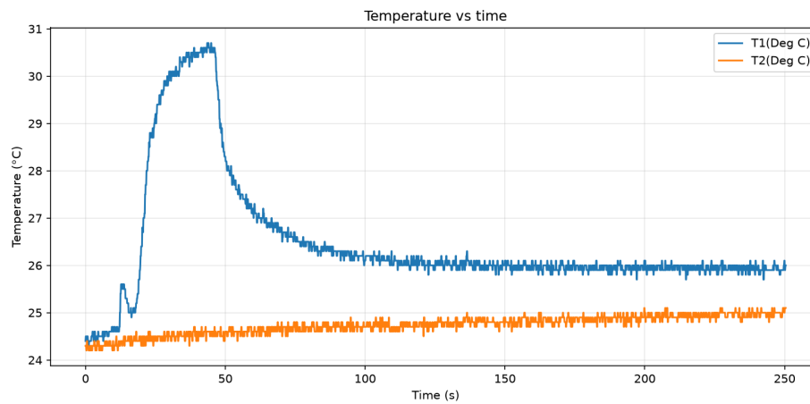
Figure 8: Tank temperature of the left tank throughout part 2.
