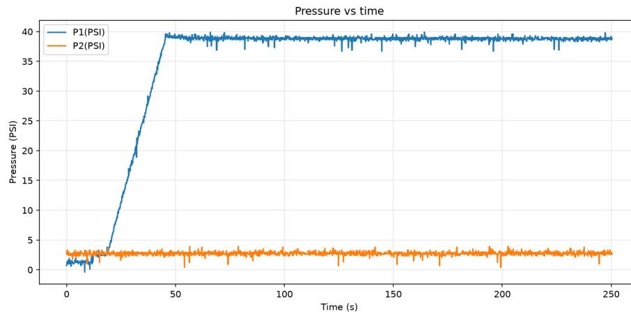
Figure 7: Tank pressure of the left tank throughout part 2.
