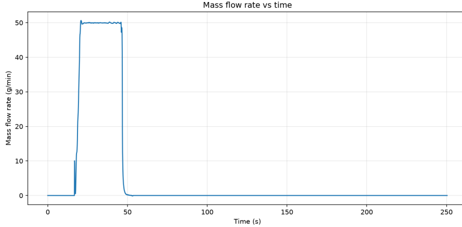
Figure 9: Mass flow rate of air into the left tank during part 2.
