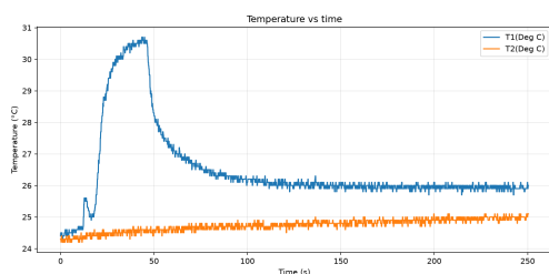
Figure 6: Tank temperatures during Part 2.
