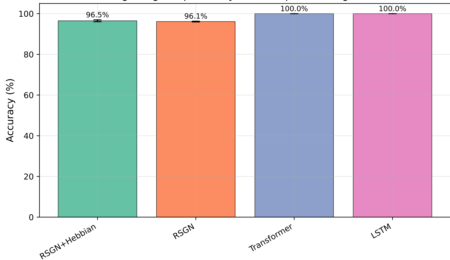
Long-Range Dependency Task (Sequence Length 128)
