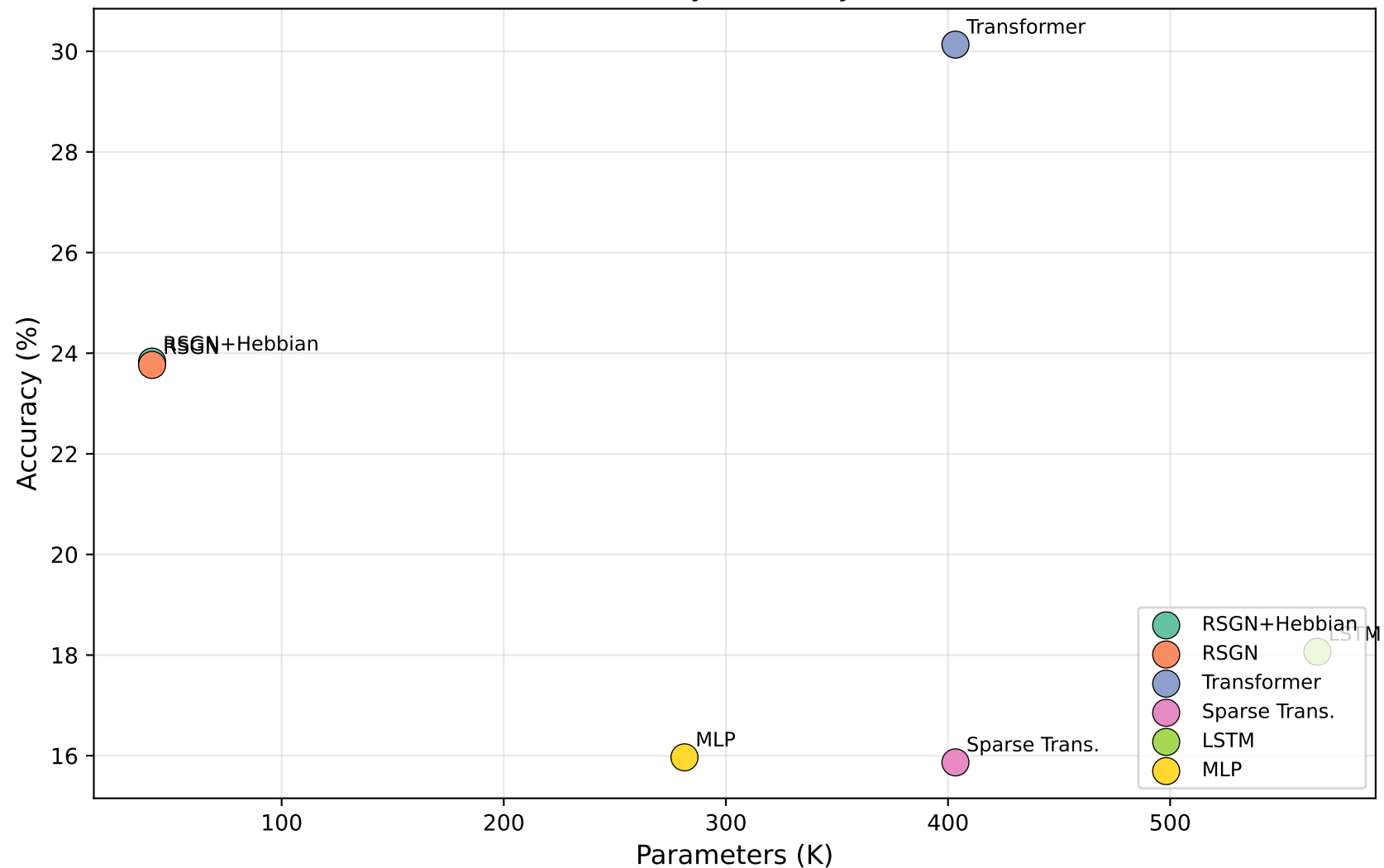
Parameter Efficiency: Accuracy vs Model Size
