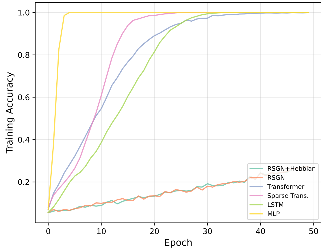
Training Curves
