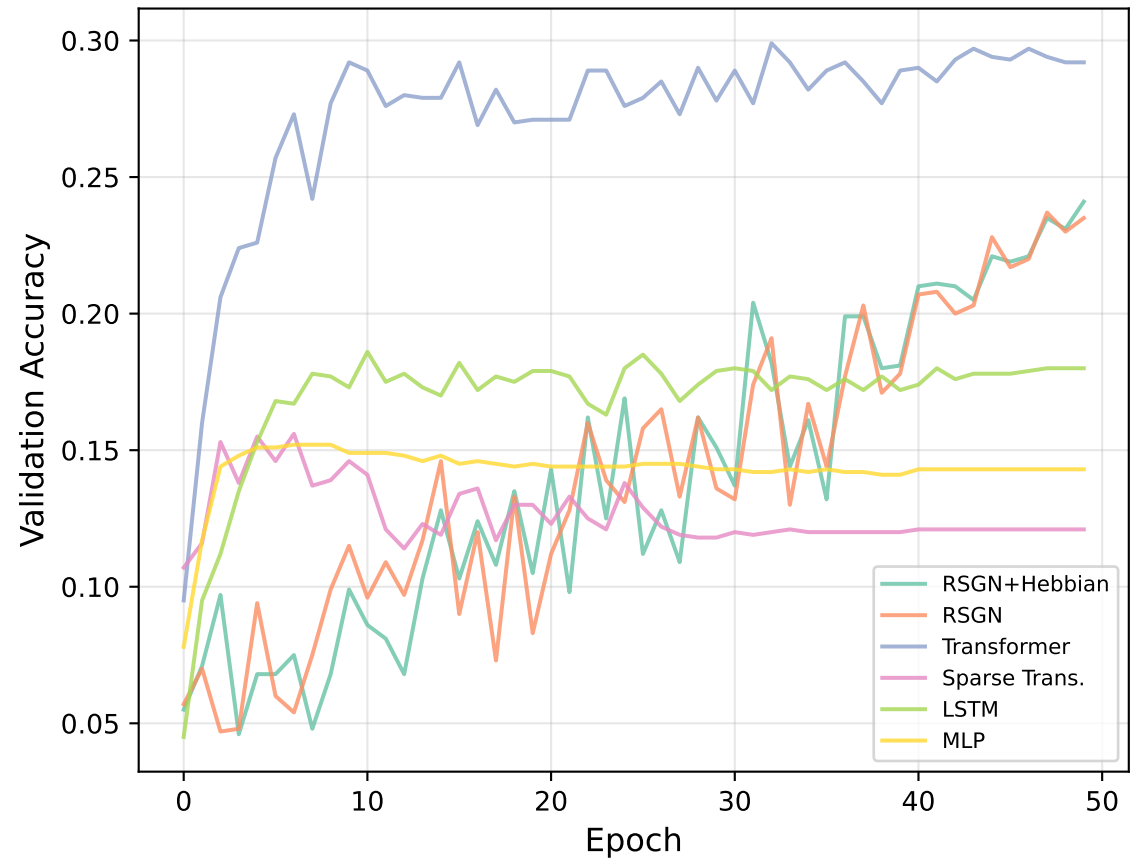
Validation Curves
