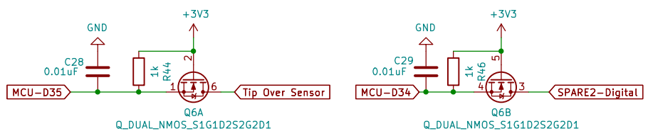
Tip Over Sensor
