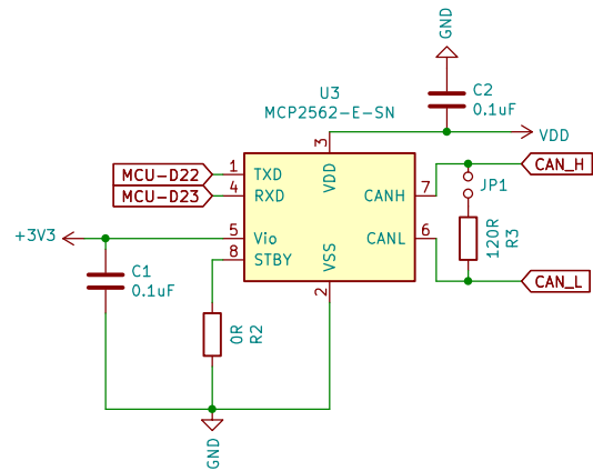
CAN Transceiver
