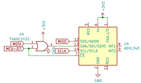
Accelerometer
