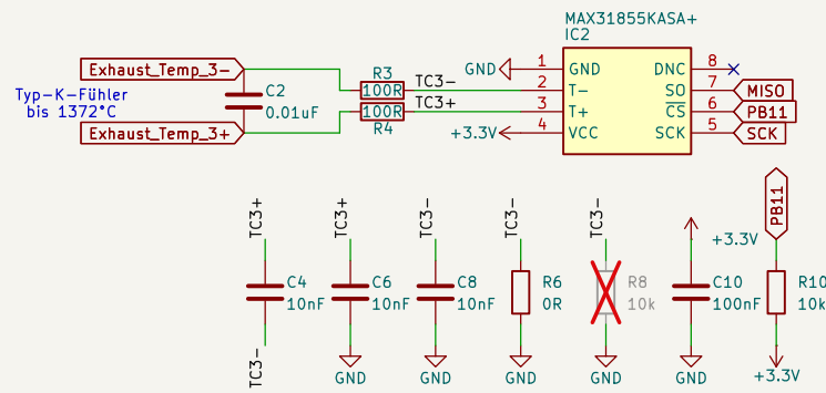
Exhaust Temp 3
