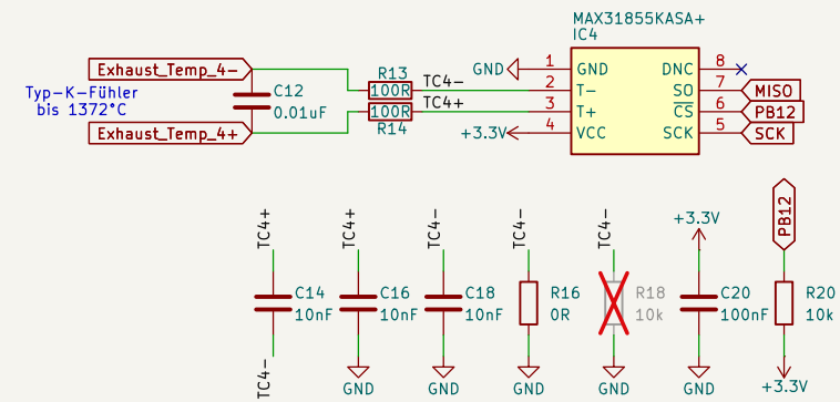
Exhaust Temp 4
