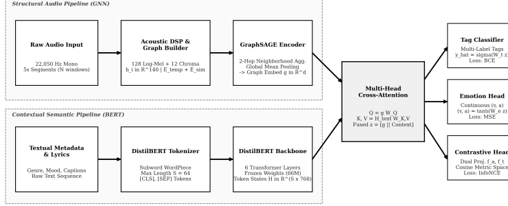
Figure 1: Overview of the Proposed Hybrid GNN-BERT Architecture. Raw audio is segmented into 5-second windows to construct a Music Structure Graph with temporal and acoustic similarity edges, processed by a GraphSAGE encoder. Concurrently, lyrics and contextual metadata are processed by DistilBERT. A multi-head cross-attention mechanism fuses structural audio features with textual tokens, driving multi-label tag classification, continuous emotion regression, and InfoNCE contrastive text-to-music retrieval.
