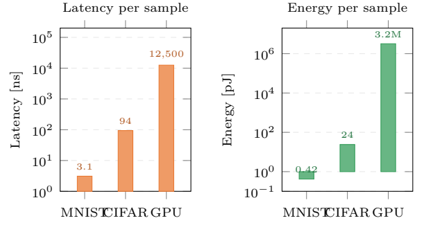
Fig. 4. Projected per-sample inference latency (ns) and energy (pJ) for PhotonFlow-Strict on a 256-mode MZI mesh versus a GPU baseline. Photonic numbers are first-principles projections from [1], [2], [14] (4-bit phase quantisation, 0.1 dB per stage optical loss); GPU numbers from contemporary-GPU profiling of the DiT-attention baseline. Both axes log scale. \dagger all photonic values are analytic projections, not measured.
