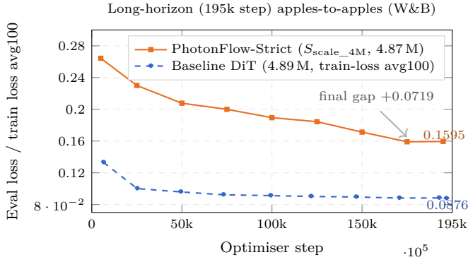
Fig. 2. 195,000-step matched-recipe trajectory. PhotonFlow-Strict descends from 0.2643 (step 5,000) to 0.1595 (step 195,000); the baseline from 0.1331 to 0.0876 over the same window. The gap widens from the 2,000-step value of +0.0629 (Sec. IV-E) to +0.0719 at 195,000 – evidence that the residual penalty at the 4.87 M scale is architectural rather than optimisation-budget.
