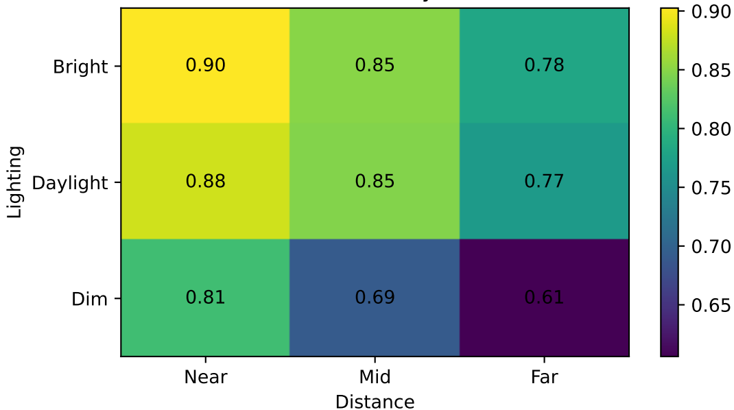
Stable ID accuracy (mean)
