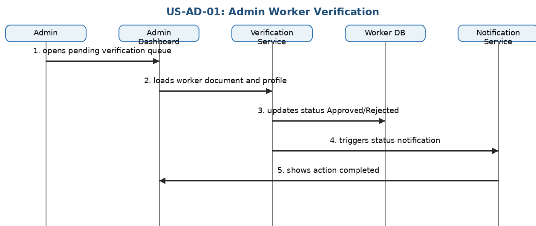
Figure 4: Sequence Diagram - Admin Worker Verification
