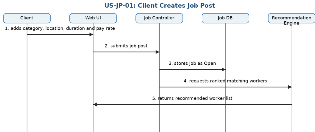
Figure 5: Sequence Diagram - Client Creates Job Post
