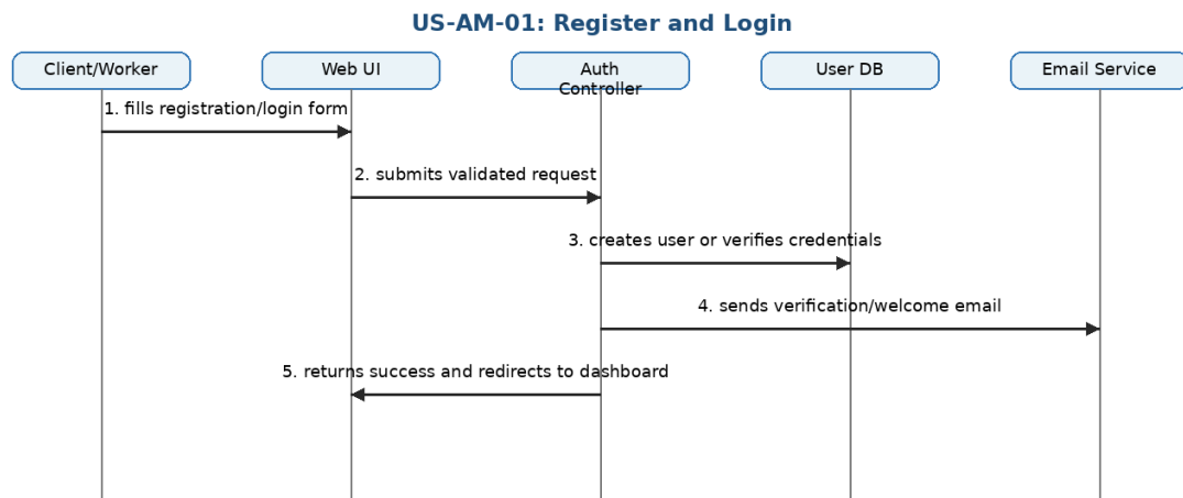
Figure 2: Sequence Diagram - Register and Login
