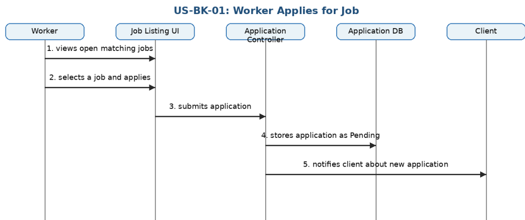
Figure 6: Sequence Diagram - Worker Applies for Job
