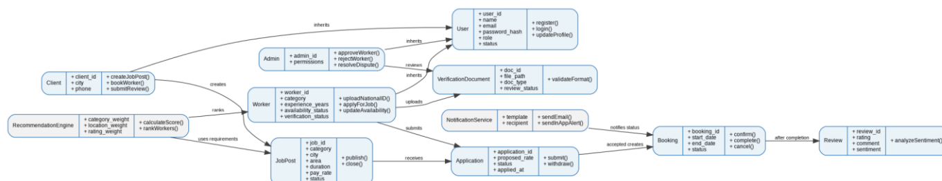
Figure 1: Sprint 1 Design Class Diagram - QuickHire Core Marketplace Classes
