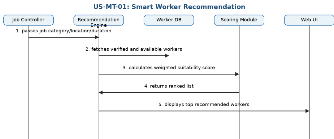
Figure 7: Sequence Diagram - Smart Worker Recommendation
