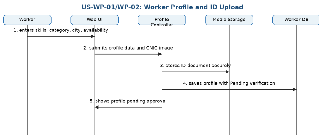
Figure 3: Sequence Diagram - Worker Profile and ID Upload
