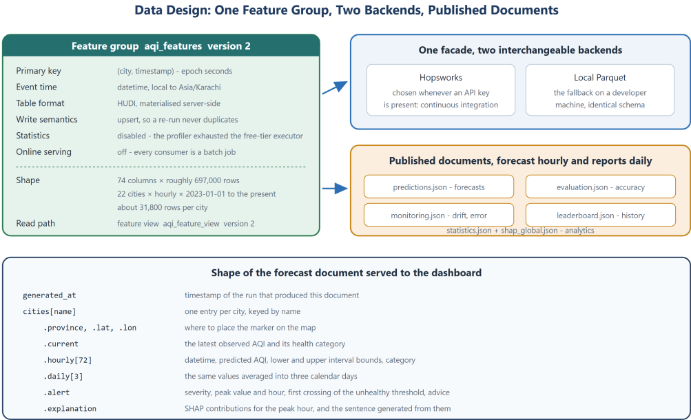
Figure 5.3: Data design: the feature group and its keys, the two interchangeable storage backends, the published documents, and the structure of the forecast payload.
