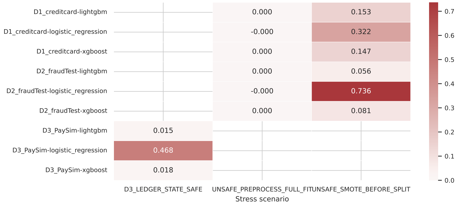
Average Precision Leakage Inflation Index
