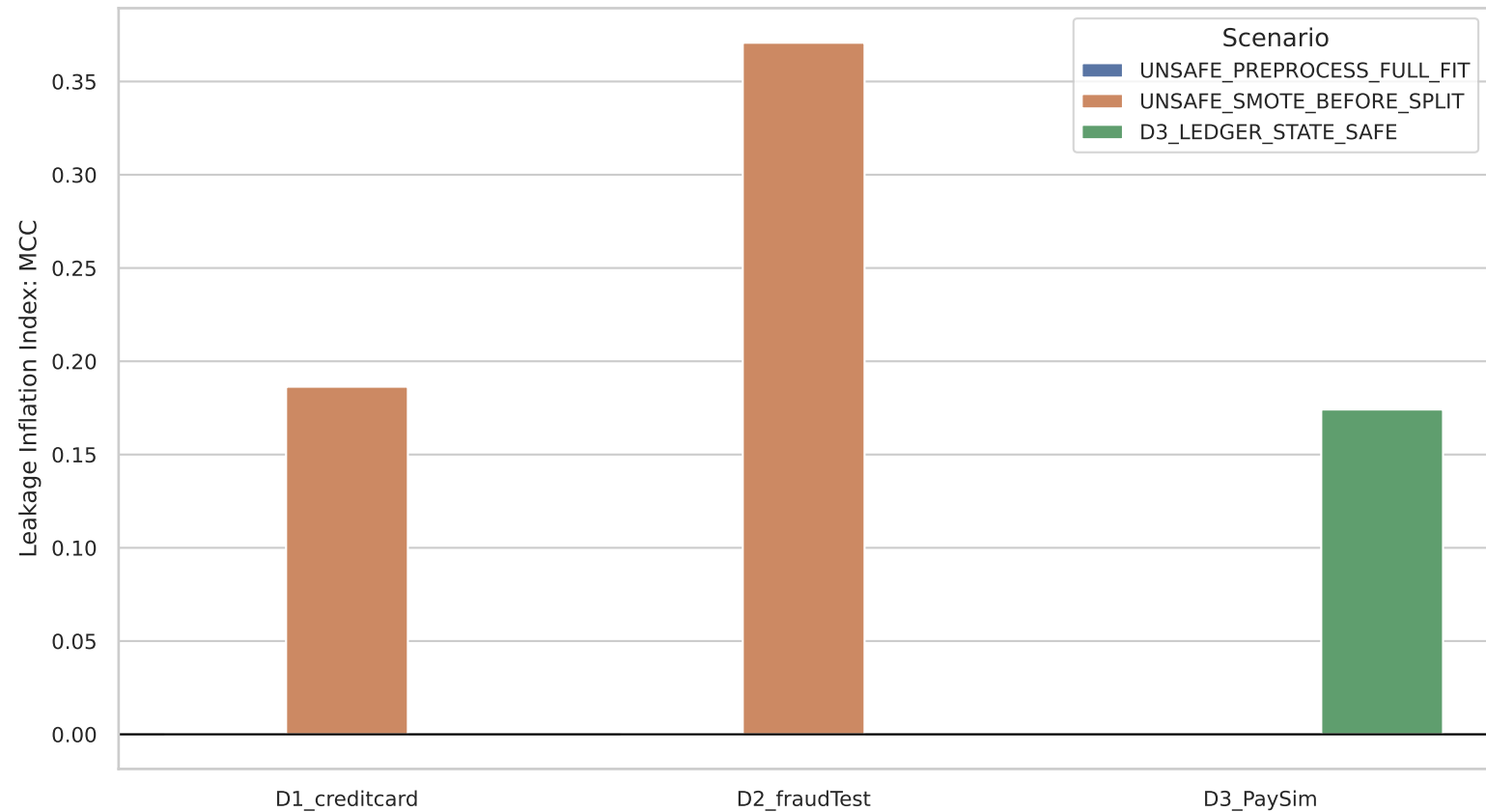
Leakage Inflation Index: MCC by Dataset and Stress Scenario
