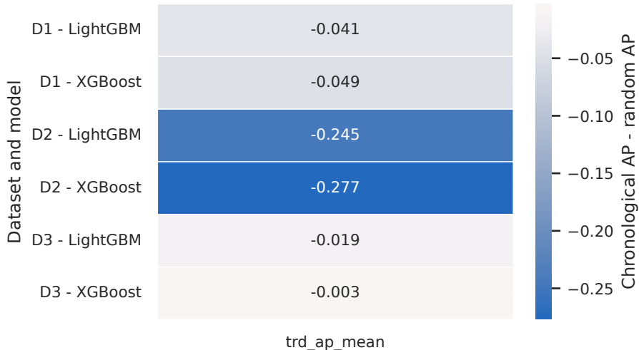
Mean Temporal Robustness Drop in AP
