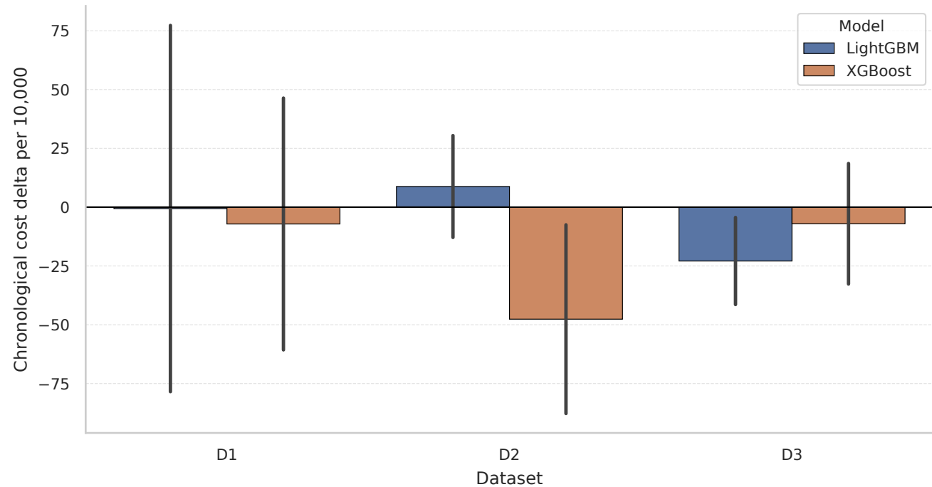
Chronological cost delta per 10,000 across five seeds
