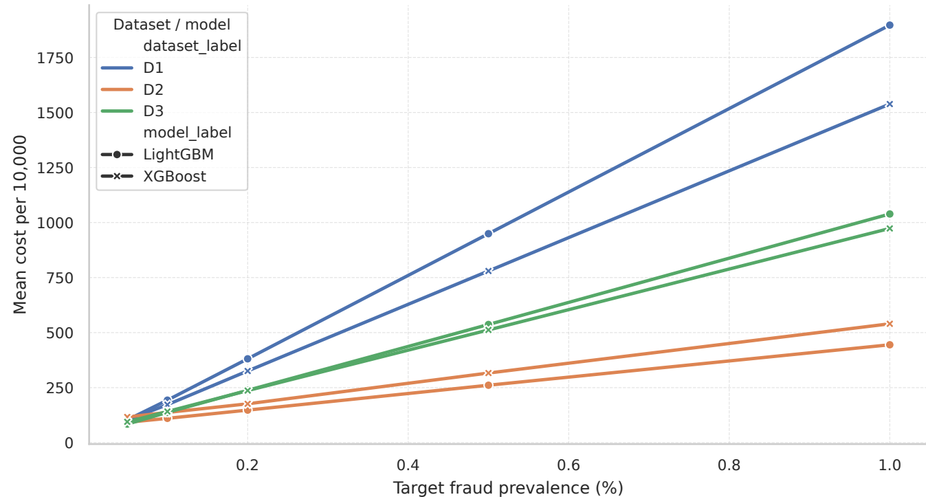
Mean cost per 10,000 under prevalence shift
