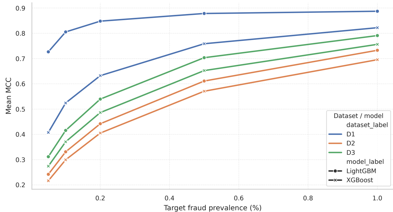
Mean MCC under prevalence shift
