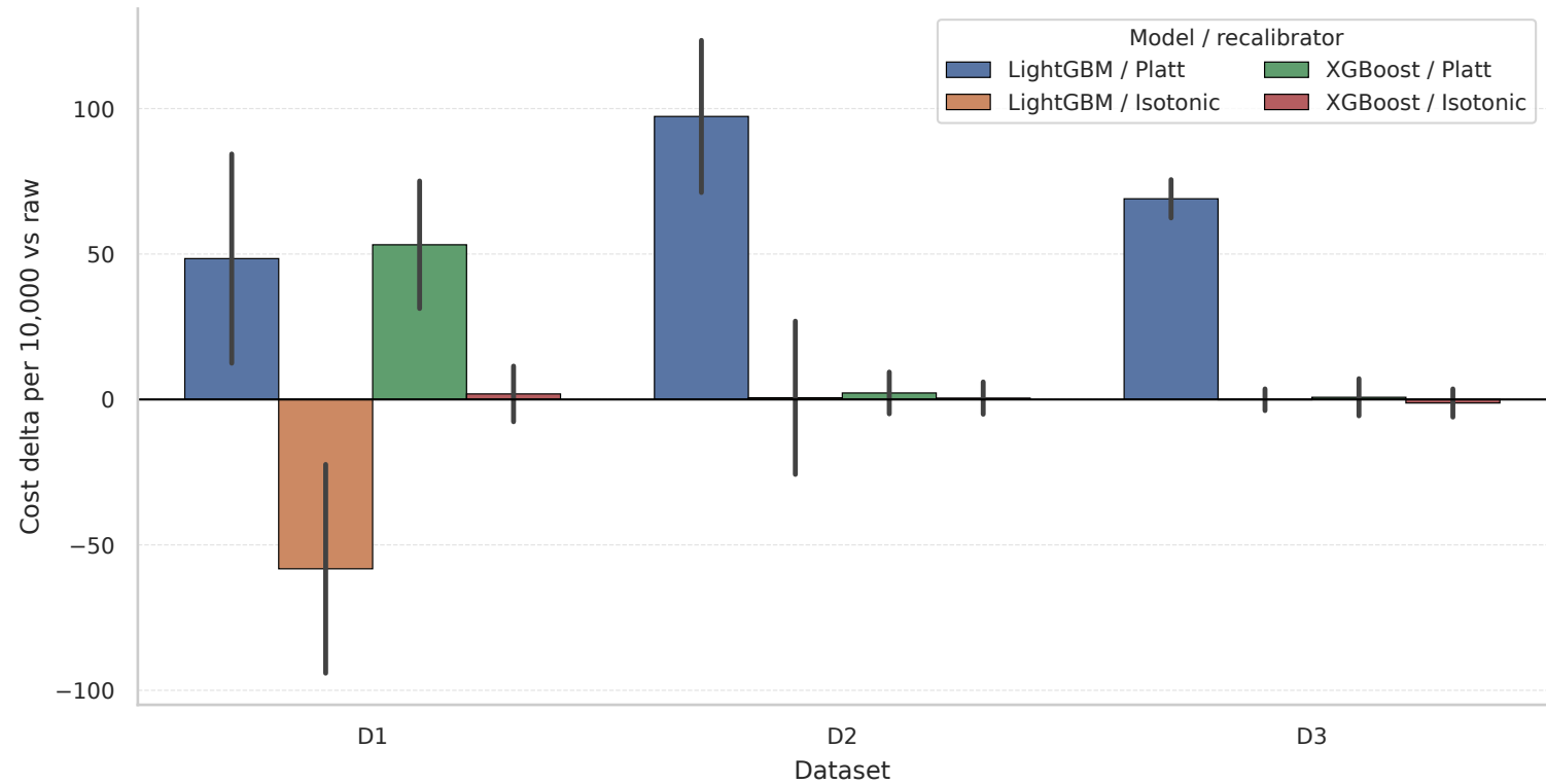
Cost delta per 10,000 vs raw across five seeds
