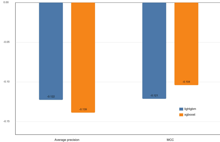
D2 Chronological Performance Delta
