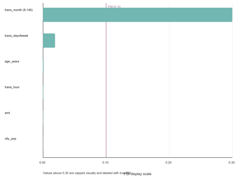
D2 Feature Drift (PSI, capped)
