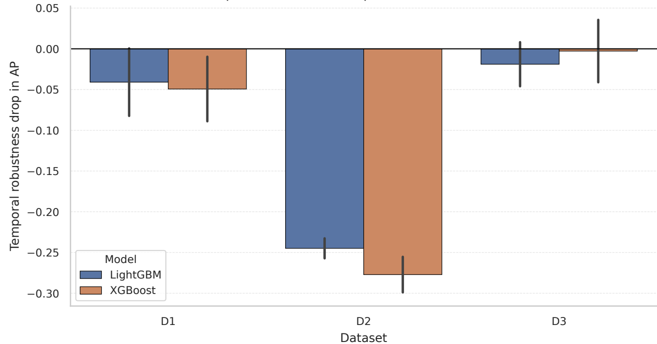
Temporal robustness drop in AP across five seeds
