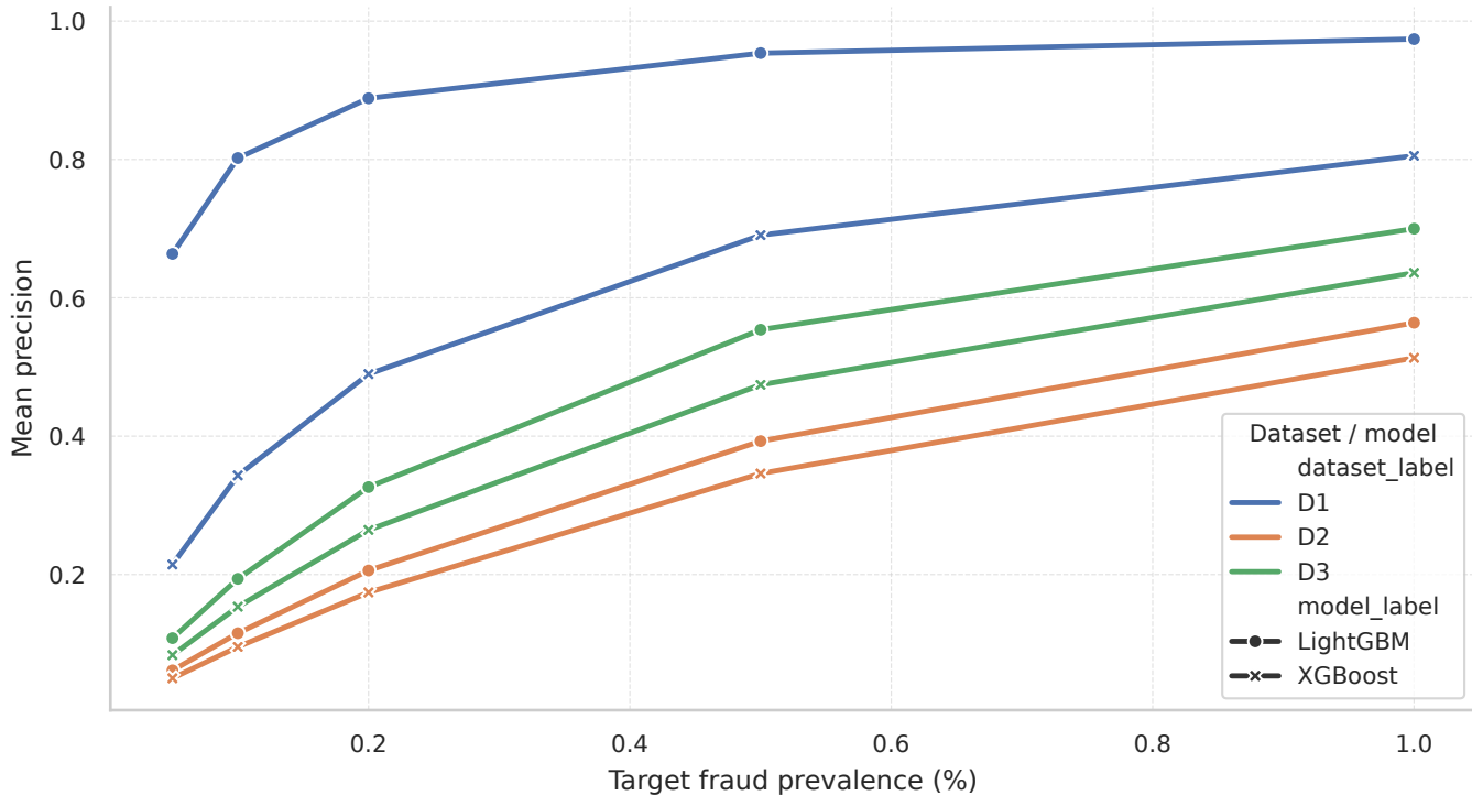
Mean precision under prevalence shift
