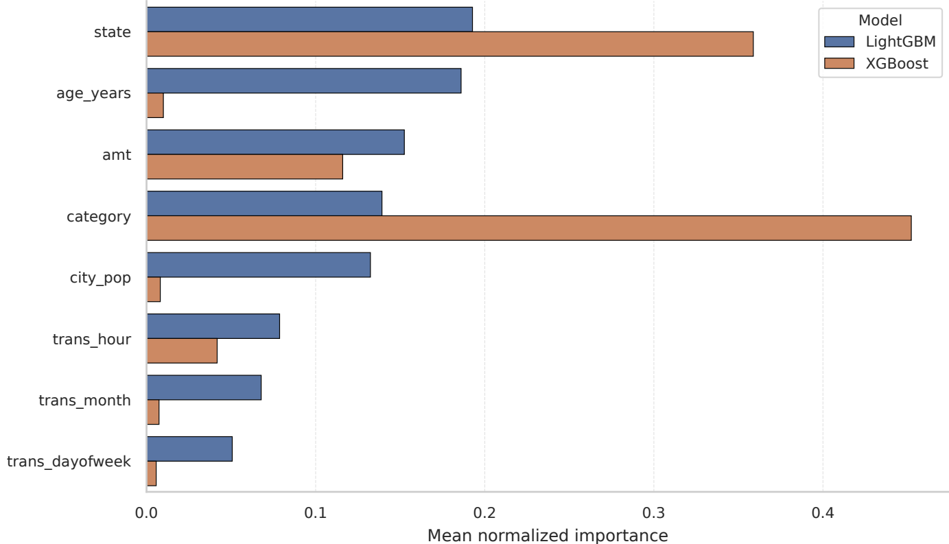
Top Strict Features: D2
