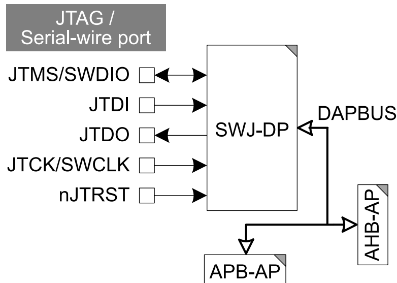
Figure 2.4: Structure of a Debug Access Port[14]
