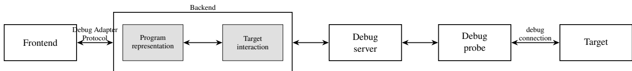
Figure 2.1: Conceptual decomposition of a debugger
