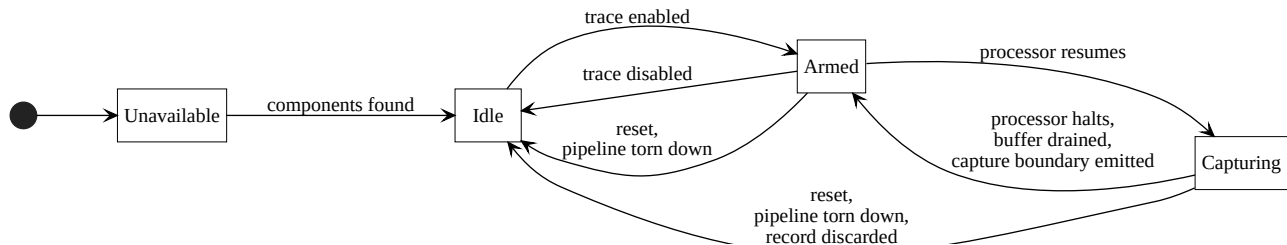
Figure 4.6: The trace lifecycle
