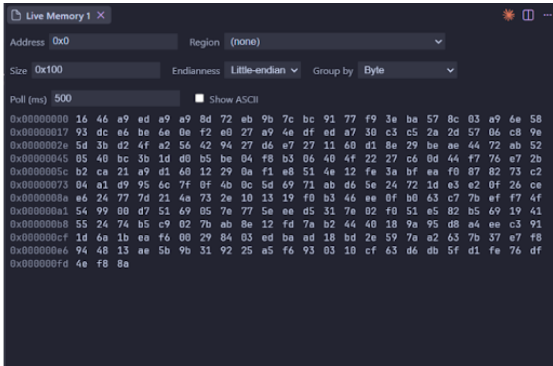
Figure 5.13: A live memory panel.
