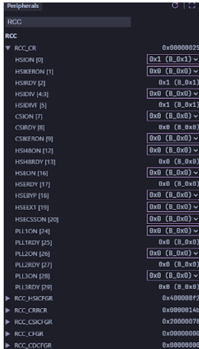
Figure 5.12: The peripheral view, with a register expanded to its individual fields.
