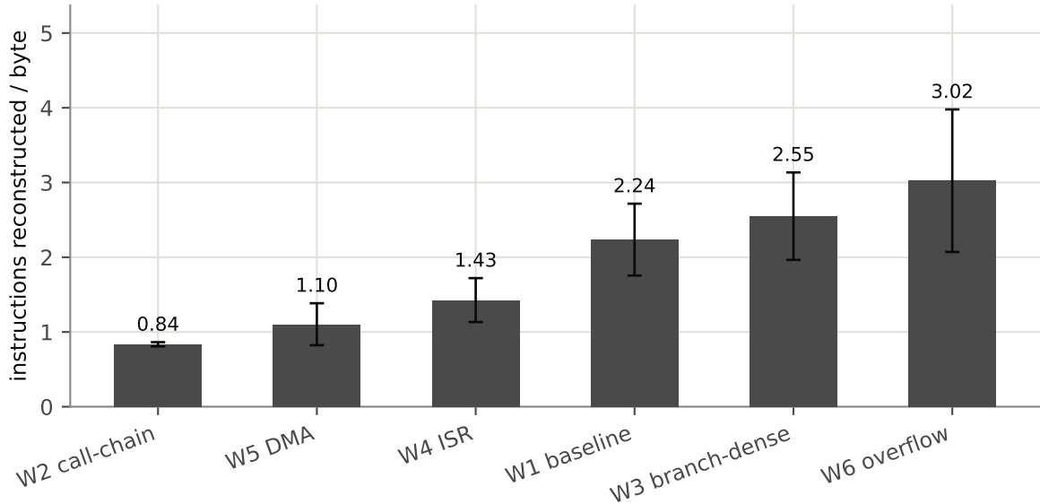
Instruction density by workload (mean \pm stdev, n=6 captures each)
