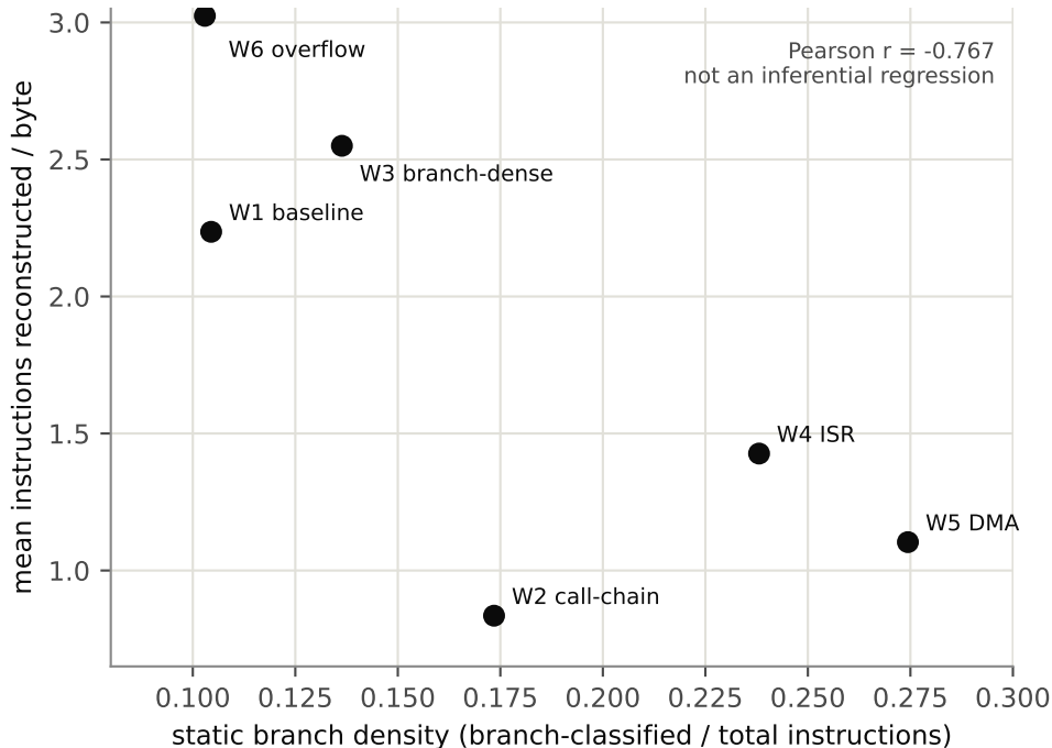
Branch density vs. instruction density (illustrative, N=6)
