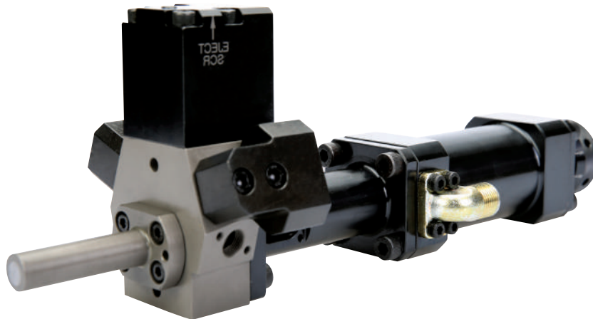
DTRC (Double Tilted Rear Chamber)
