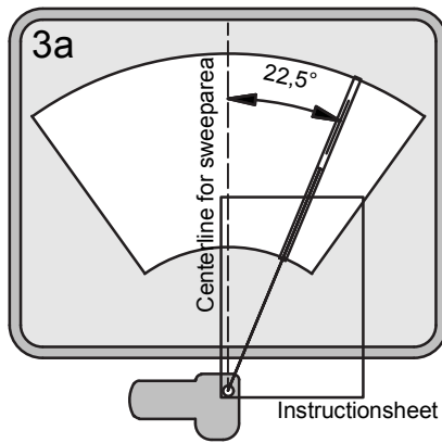
Standard arm
