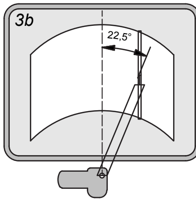
Pantograph arm
