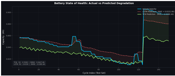
Fig. 6. Comparison of Actual vs. Predicted Capacity for a representative test-set battery, demonstrating tracking of degradation trajectory across the evaluated test cycles.
