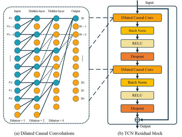
Fig. 3. Temporal Convolutional Network (TCN) layers showing dilated causal convolutions and residual blocks.
