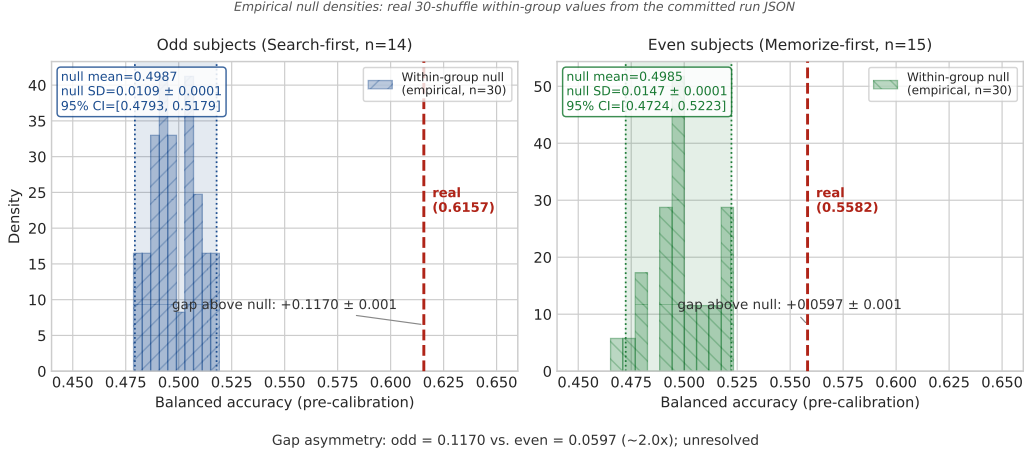
Figure 4: D2 parity-split replication: pre-calibration balanced accuracy for odd (Search-first, n=14 , 0.6157 \pm 0.001 ) and even (Memorize-first, n=15 , 0.5582 \pm 0.001 ) subject subgroups against each subgroup’s own within-group shuffled-label null (empirical, the real 30 per-shuffle values from each subgroup’s own committed run record). Both subgroups clear their own 95% CI. The gap above each subgroup’s null mean is asymmetric: 0.1170 \pm 0.001 (odd) vs. 0.0597 \pm 0.001 (even), roughly 2 \times , unresolved (§5).
