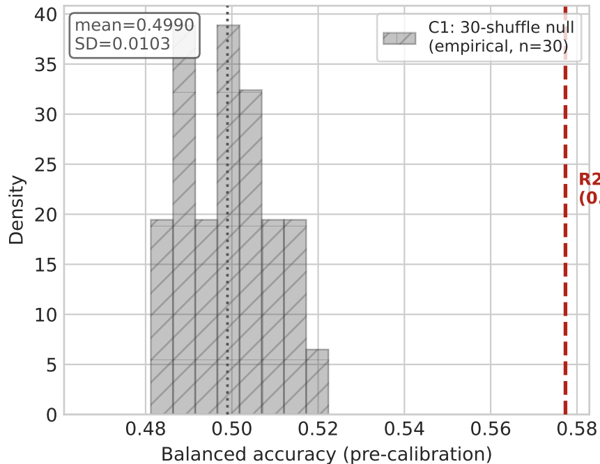
Empirical null densities: real per-shuffle values from the committed run JSONs
