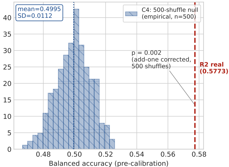
Empirical null densities: real per-shuffle values from the committed run JSONs
