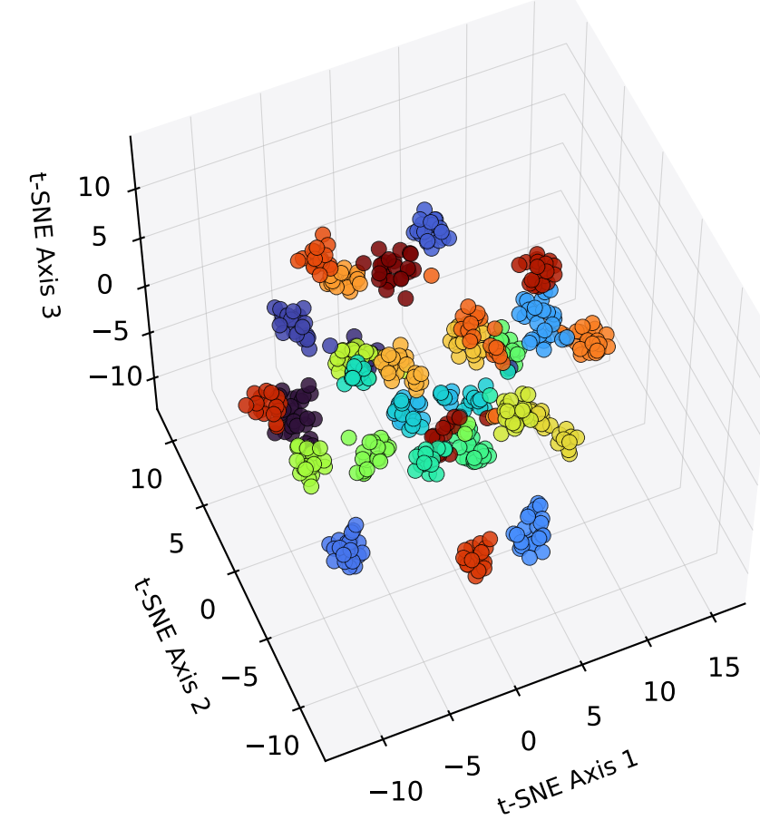
C. Same Coordinates, Colored by Subject ID (29 subjects -> geometry tracks identity, not class)
