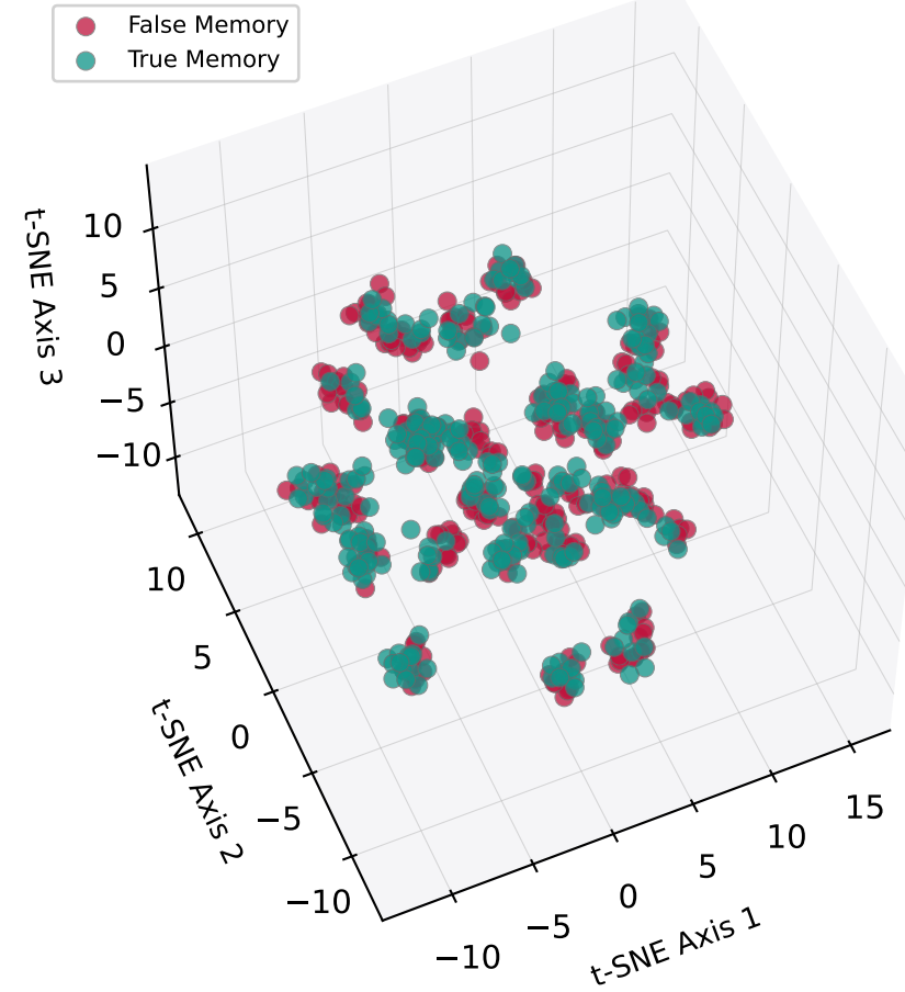
B. Multi-Subject (N=600), Colored by Class (label-informed axes; centroid gap=1.22)
