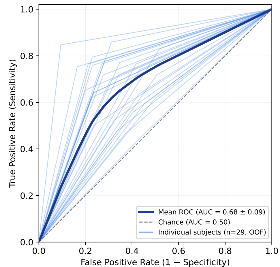
B. ROC Curve Analysis (Condition 4, Leave-One-Subject-Out, N=29)
