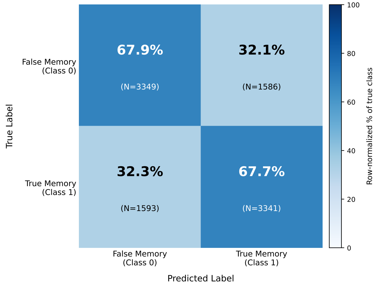
A. Aggregated Confusion Matrix (Condition 4, Out-of-Fold, Row-Normalized)
