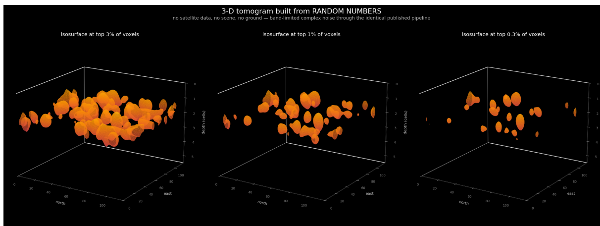
Figure 6. Three-dimensional isosurface rendering of a volume built from band-limited complex noise — no satellite data, no scene, no ground — through the identical pipeline, at three thresholds. Discrete solid bodies in a shallow slab. This is what the artifact looks like rendered in three dimensions, and it is not what the published figures look like.
