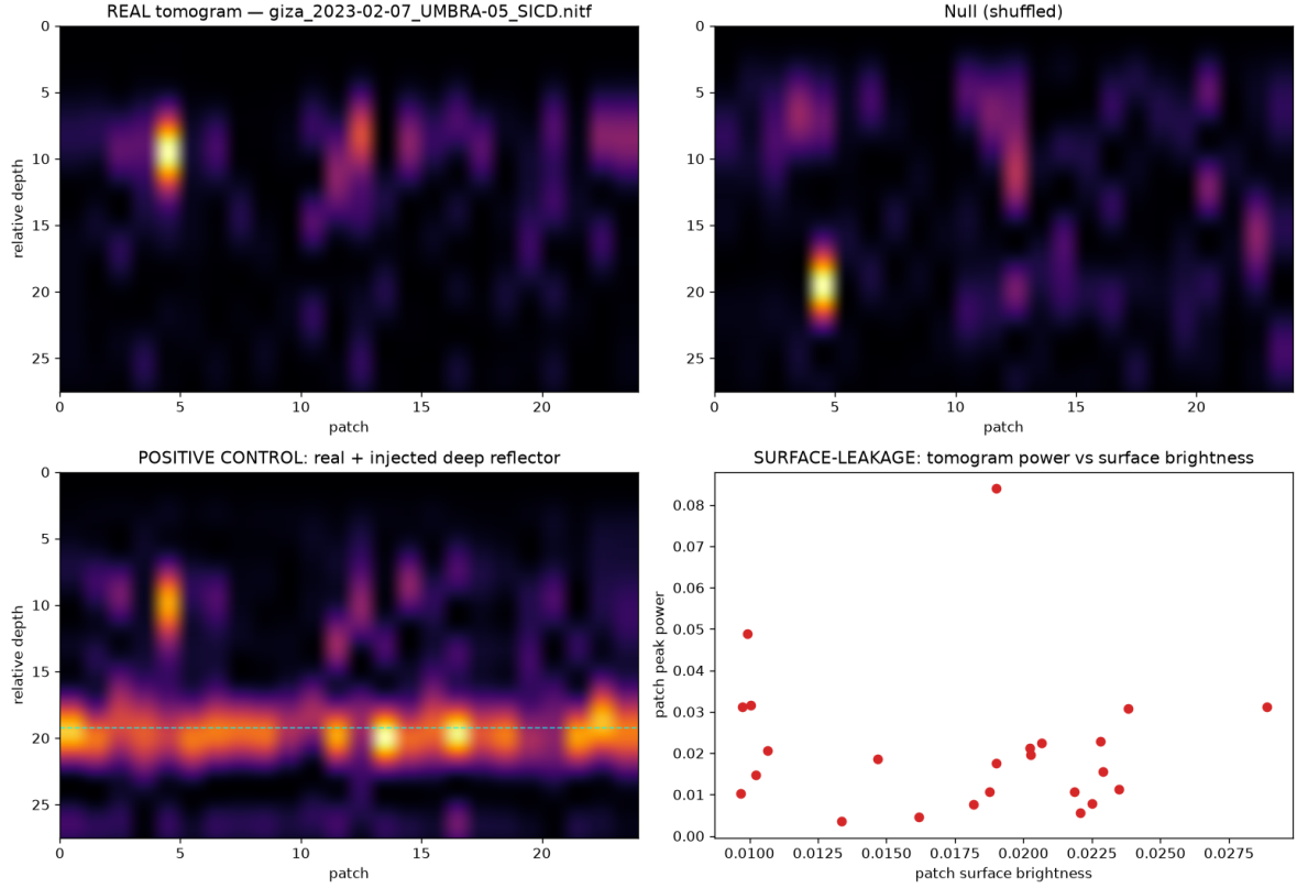
Figure 4. Giza plateau, 11 sub-apertures. Top left: the real tomogram. Top right: the same data with look order shuffled — pure noise. The two are visually indistinguishable. Bottom left: the positive control, a synthetic reflector injected at relative depth 20, which produces a continuous horizontal band across every patch at one depth — what a coherent subsurface reflector looks like. The real panel contains nothing of the kind. Bottom right: tomogram power against surface brightness, correlation 0.07 — the depth product is not surface-driven.
