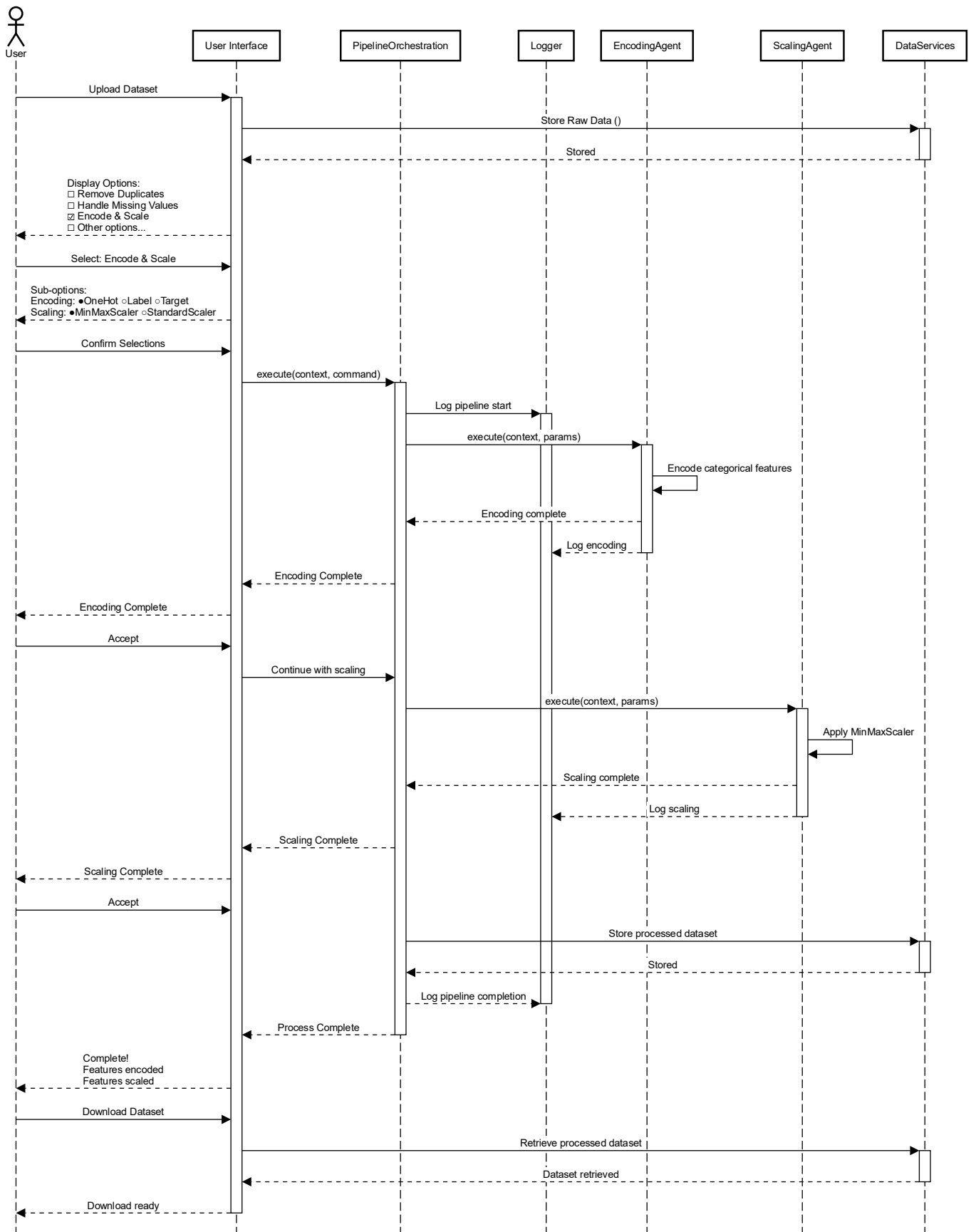
Figure 4-13 Full Automation Sequence Diagram
