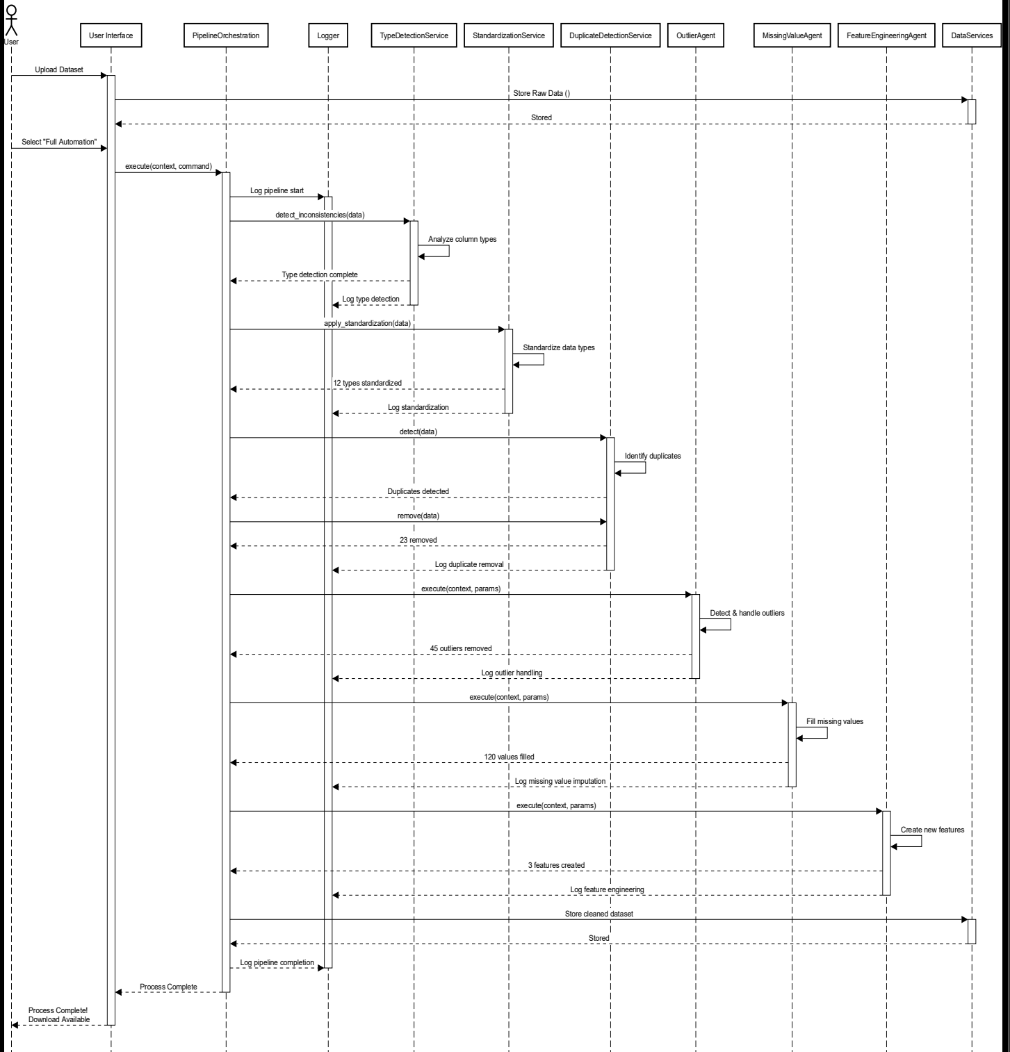
Figure 4-12 Full Automation Sequence Diagram
