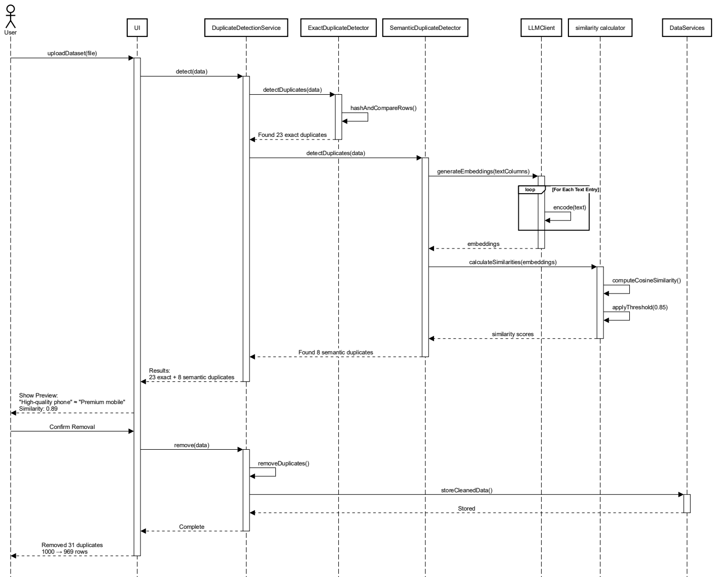
Figure 4-14 Duplicate Removal Sequence Diagram
