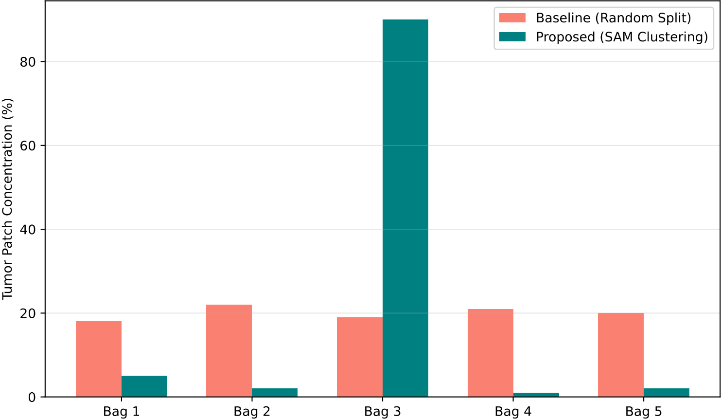
Gap 1 Analysis: Solving Tumor Dilution in Pseudo-Bags
