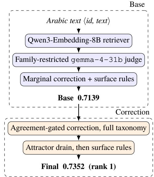
Figure 1: System overview. A Qwen3 retriever gates a broad family and a gemma-4-31b judge scores its siblings setwise; rules and an Interactive-recall pass complete the base (0.7139). GPT-5.6 and Gemini-3.6, shown all 74 definitions, then change a label only where they agree, and an attractor drain follows (0.7352, rank 1).
