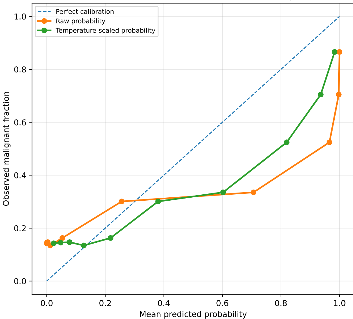
Calibration on TN3K/TNCD: ConvNeXt-Tiny
