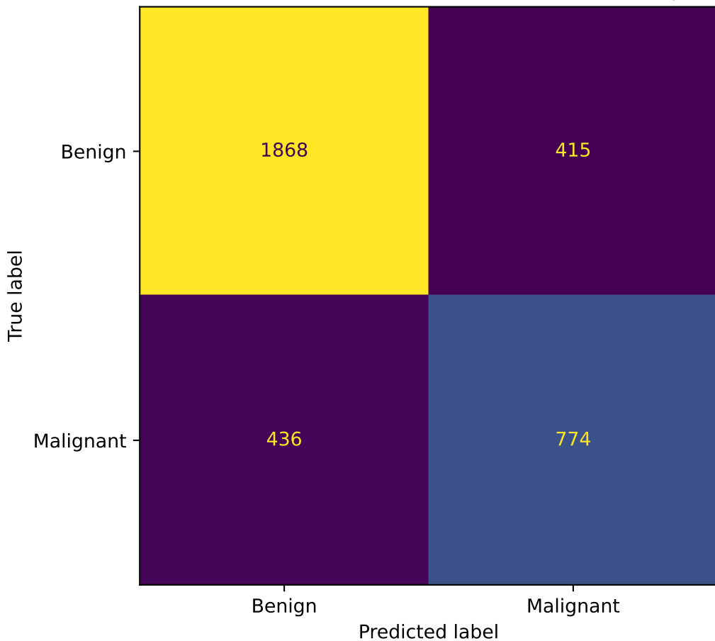
TN3K/TNCD confusion matrix: ConvNeXt-Tiny
