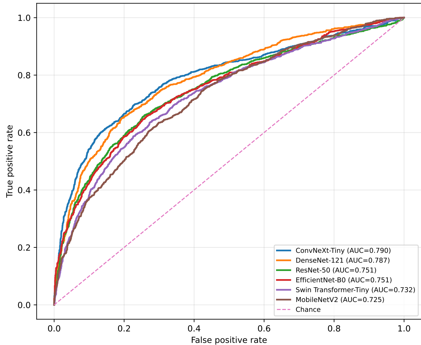
External ROC curves on TN3K/TNCD
