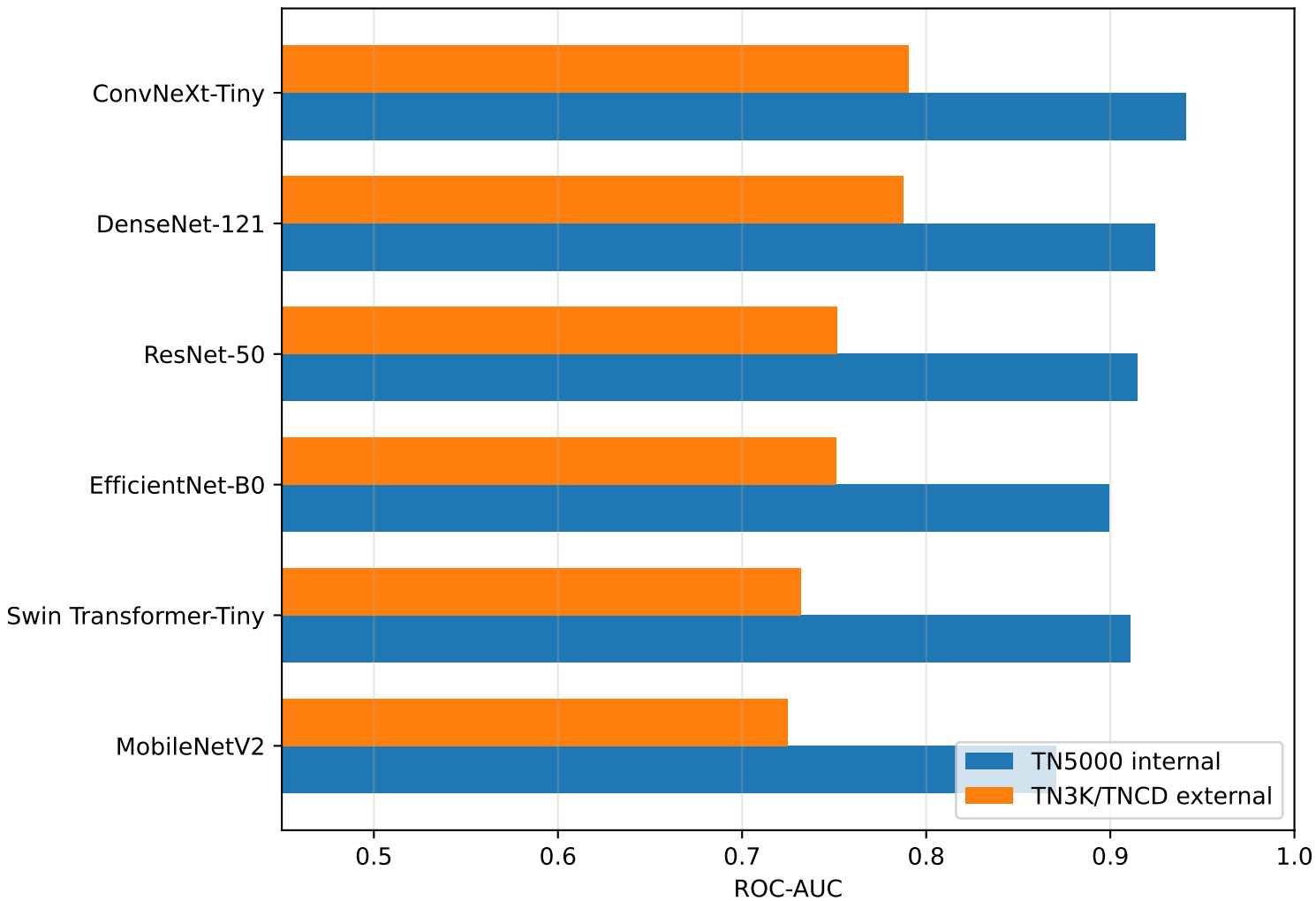
Internal vs external ROC-AUC
